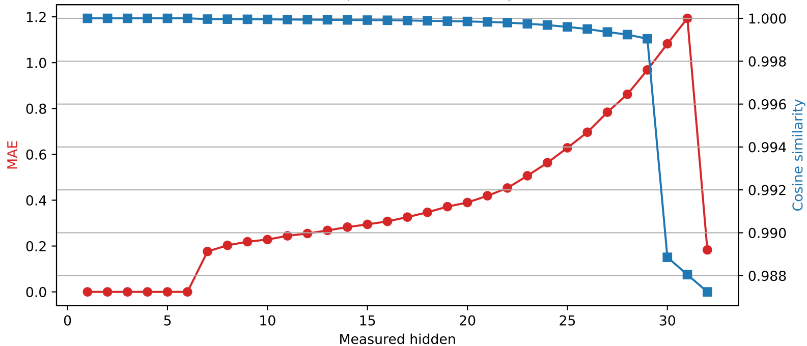
Phi-3-mini-4k-instruct | Quantized layer 6 | float16 \rightarrow int4
