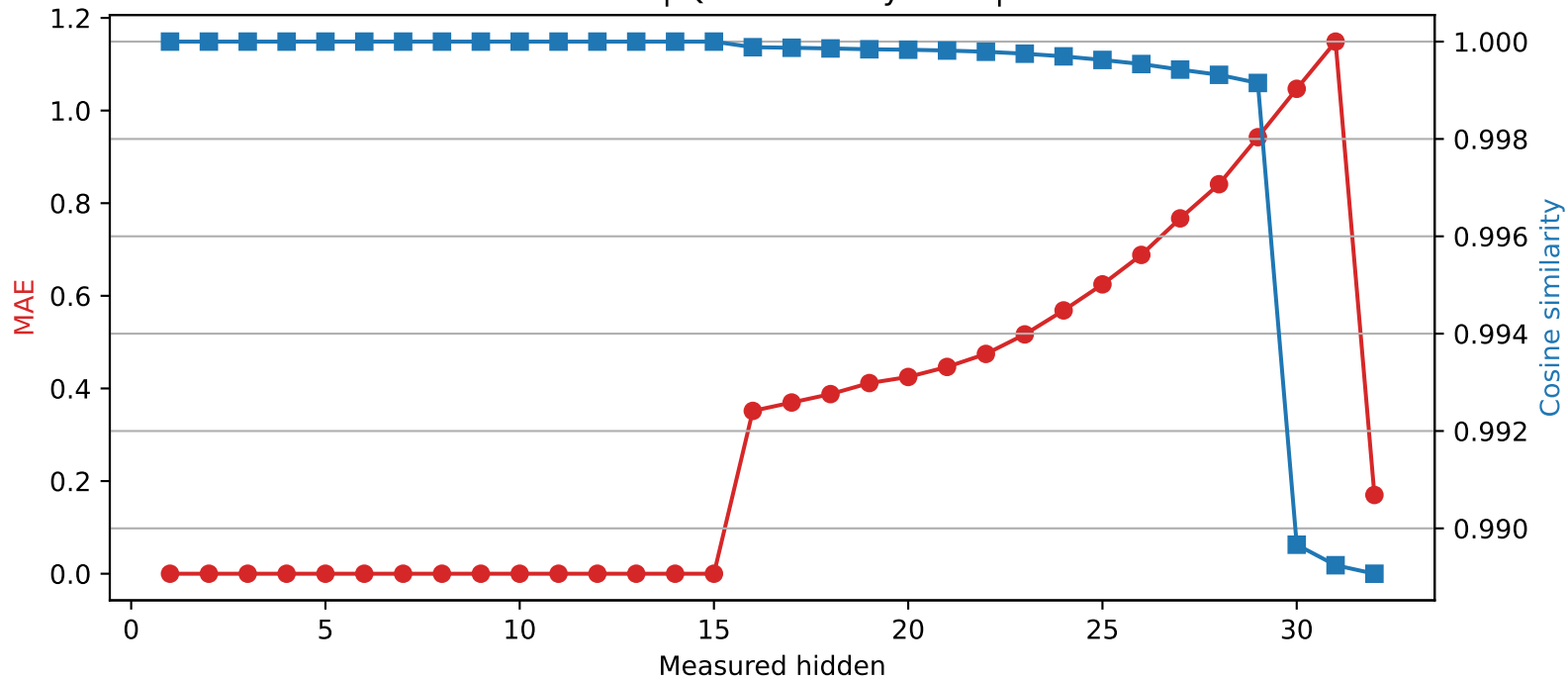
Phi-3-mini-4k-instruct | Quantized layer 15 | float16 \rightarrow int4
