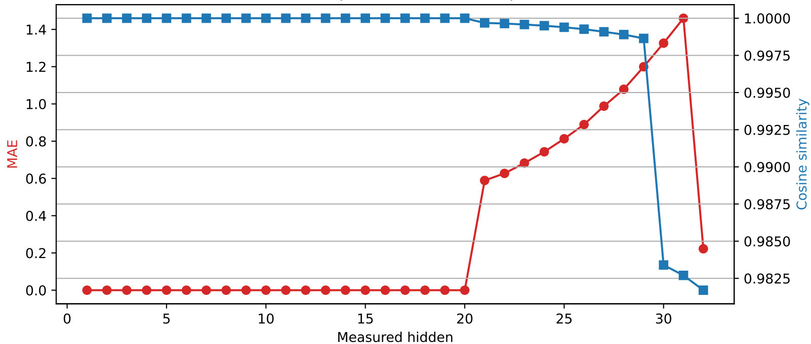
Phi-3-mini-4k-instruct | Quantized layer 20 | float16 → int4
