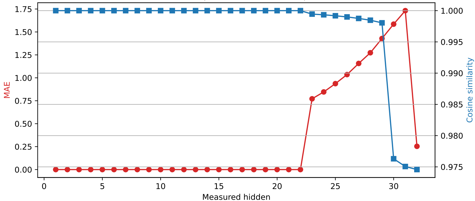
Phi-3-mini-4k-instruct | Quantized layer 22 | float16 \rightarrow int4
