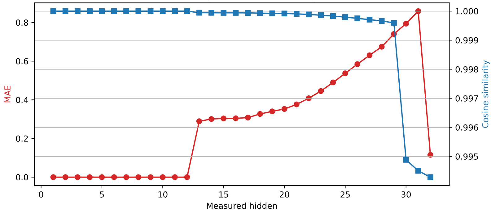
Phi-3-mini-4k-instruct | Quantized layer 12 | float16 \rightarrow int4
