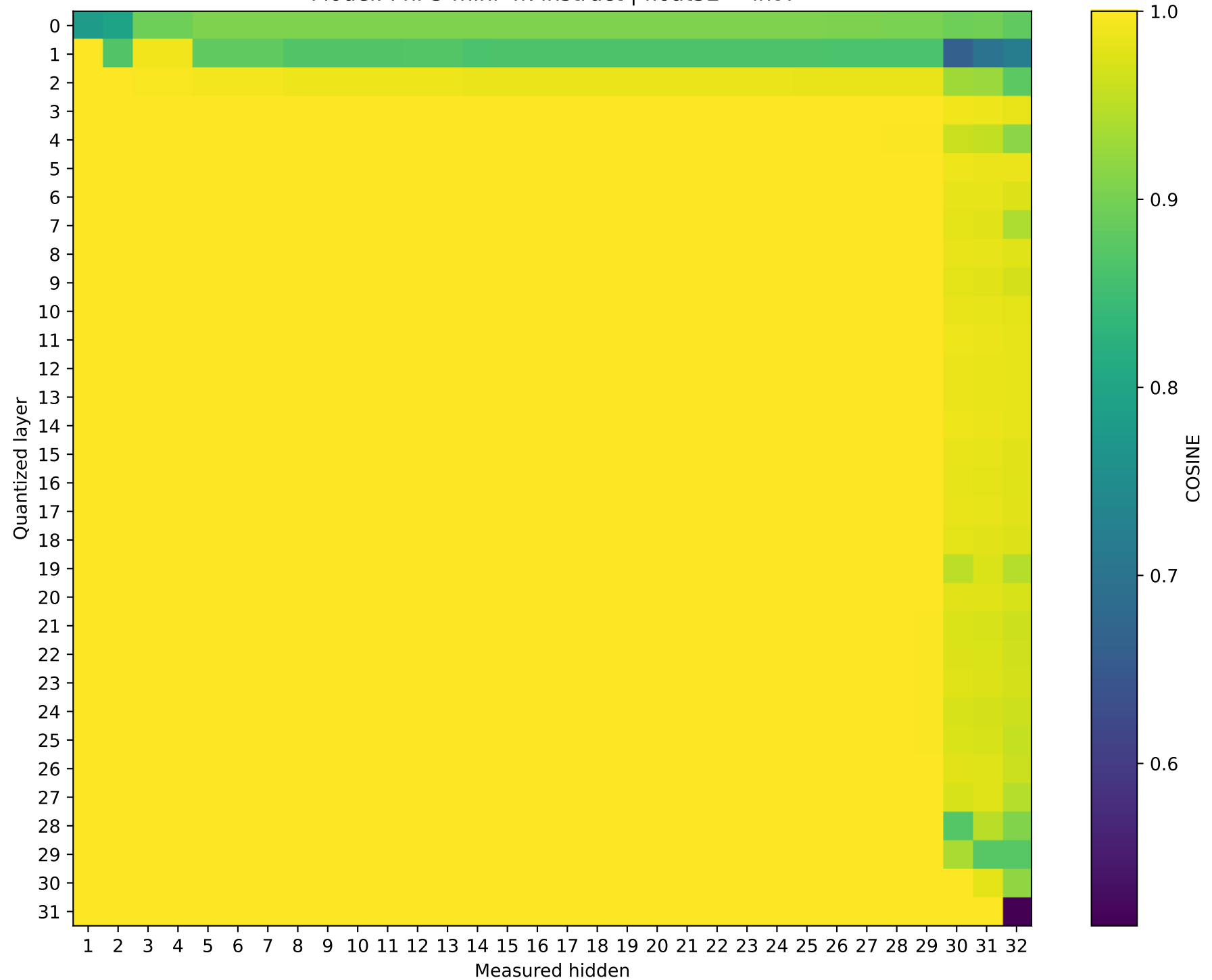
Model: Phi-3-mini-4k-instruct | float32 → int4
