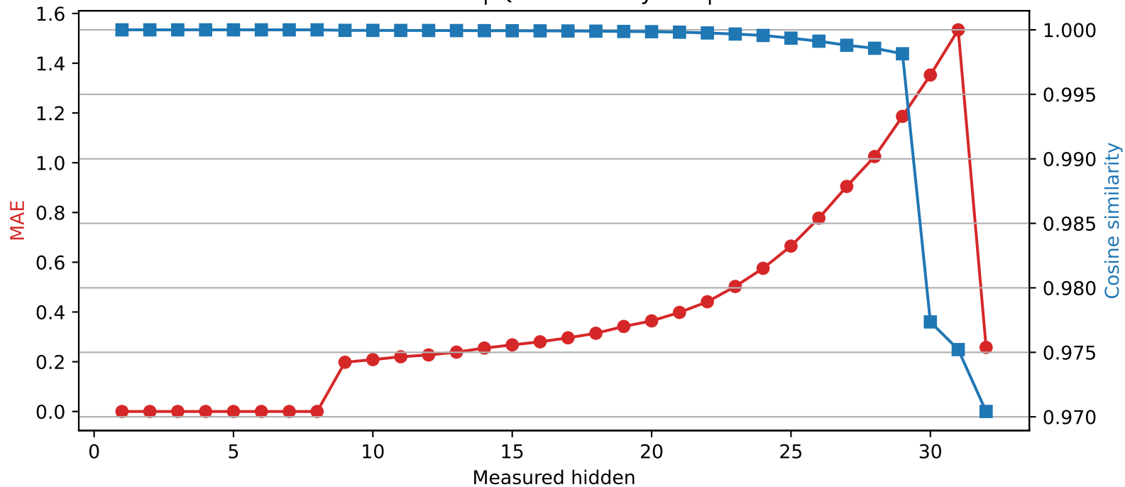
Phi-3-mini-4k-instruct | Quantized layer 8 | float32 \rightarrow int4
