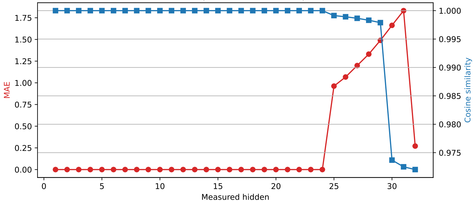
Phi-3-mini-4k-instruct | Quantized layer 24 | float32 \rightarrow int4
