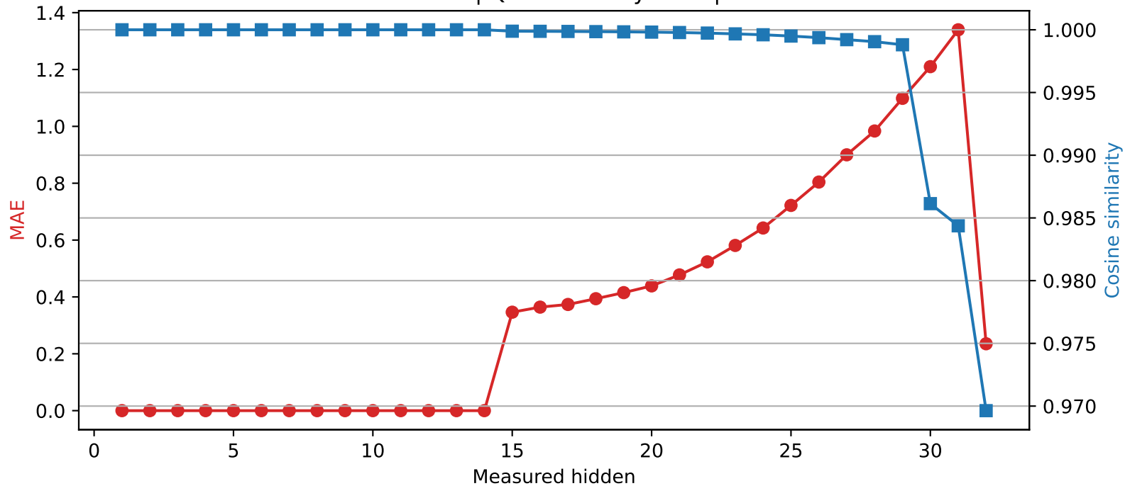
Phi-3-mini-4k-instruct | Quantized layer 14 | float32 \rightarrow int4
