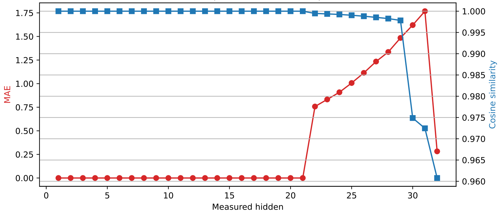
Phi-3-mini-4k-instruct | Quantized layer 21 | float32 → int4
