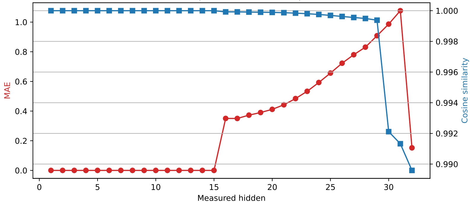
Phi-3-mini-4k-instruct | Quantized layer 15 | float32 → int4
