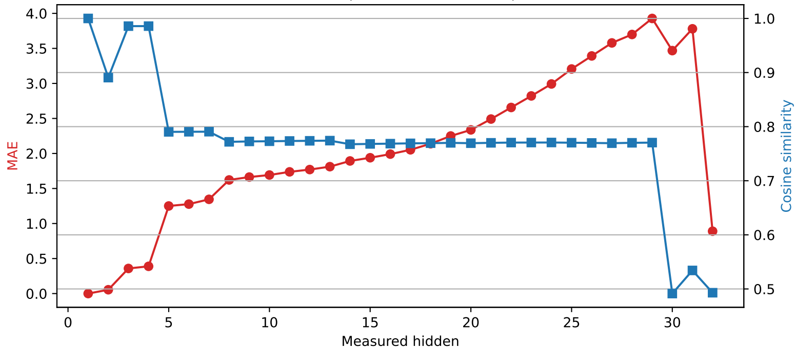
Phi-3-mini-4k-instruct | Quantized layer 1 | float64 → int4
