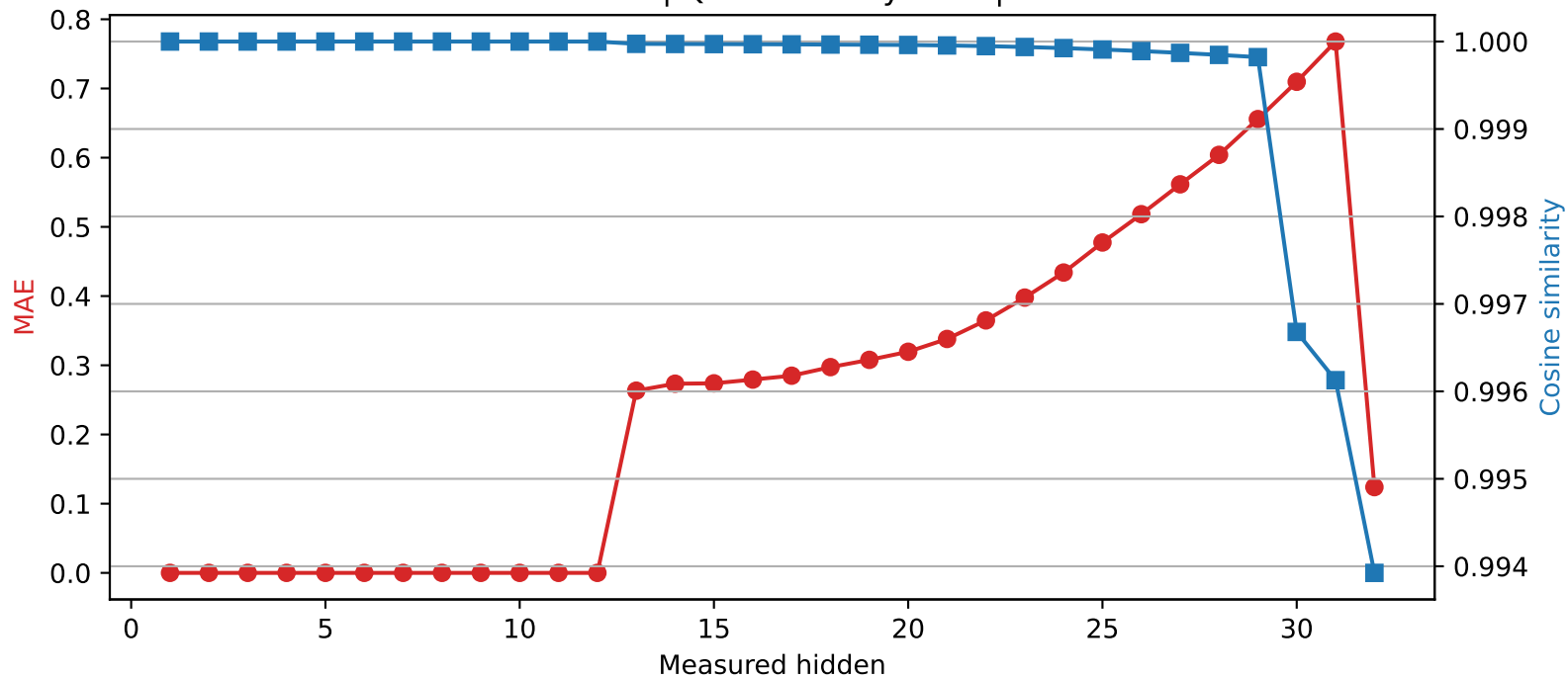
Phi-3-mini-4k-instruct | Quantized layer 12 | float64 → int4
