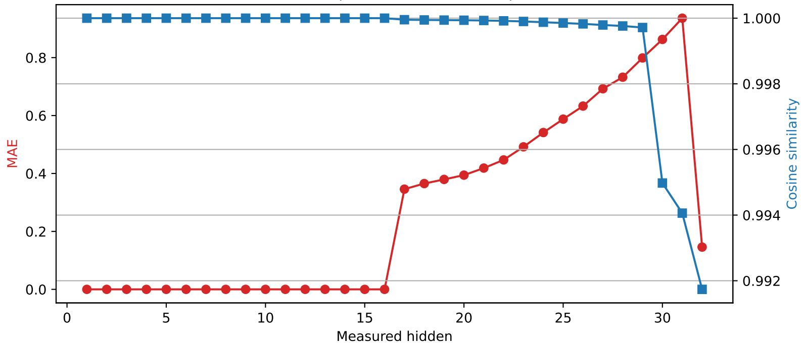
Phi-3-mini-4k-instruct | Quantized layer 16 | float64 → int4
