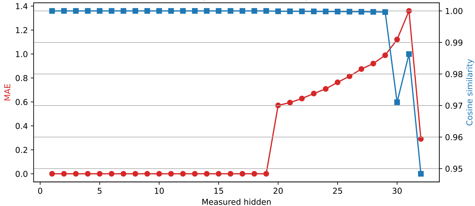
Phi-3-mini-4k-instruct | Quantized layer 19 | float64 \rightarrow int4
