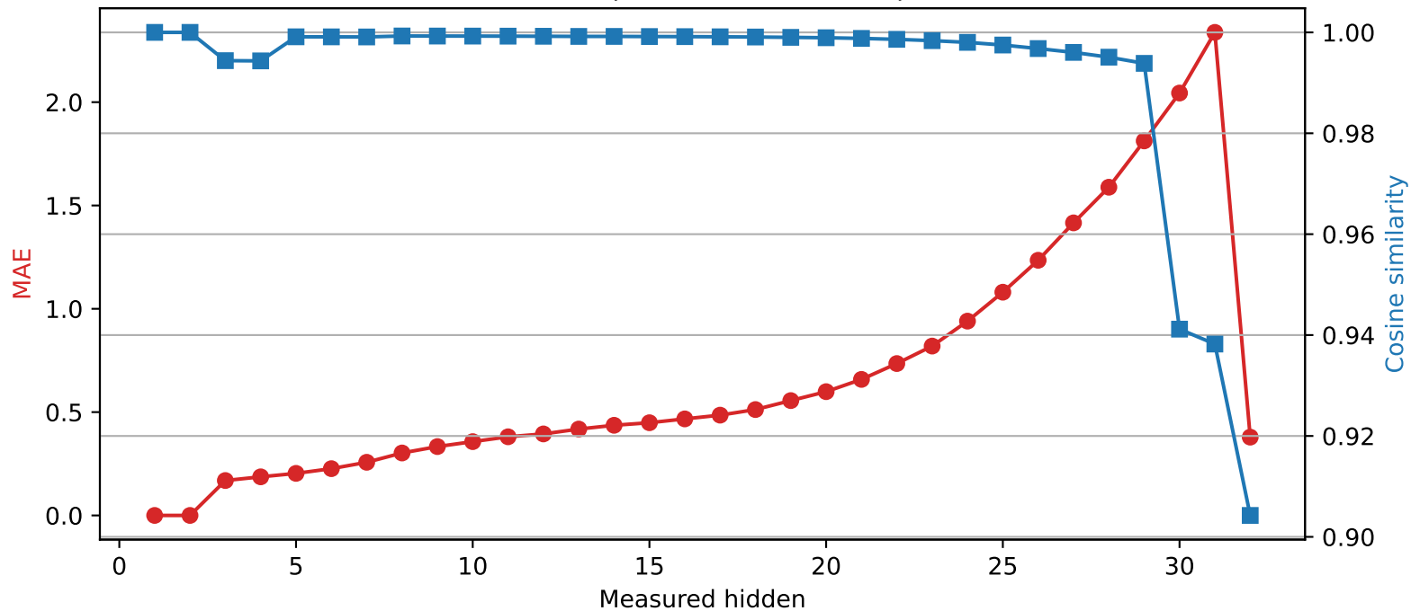
Phi-3-mini-4k-instruct | Quantized layer 2 | float64 → int4
