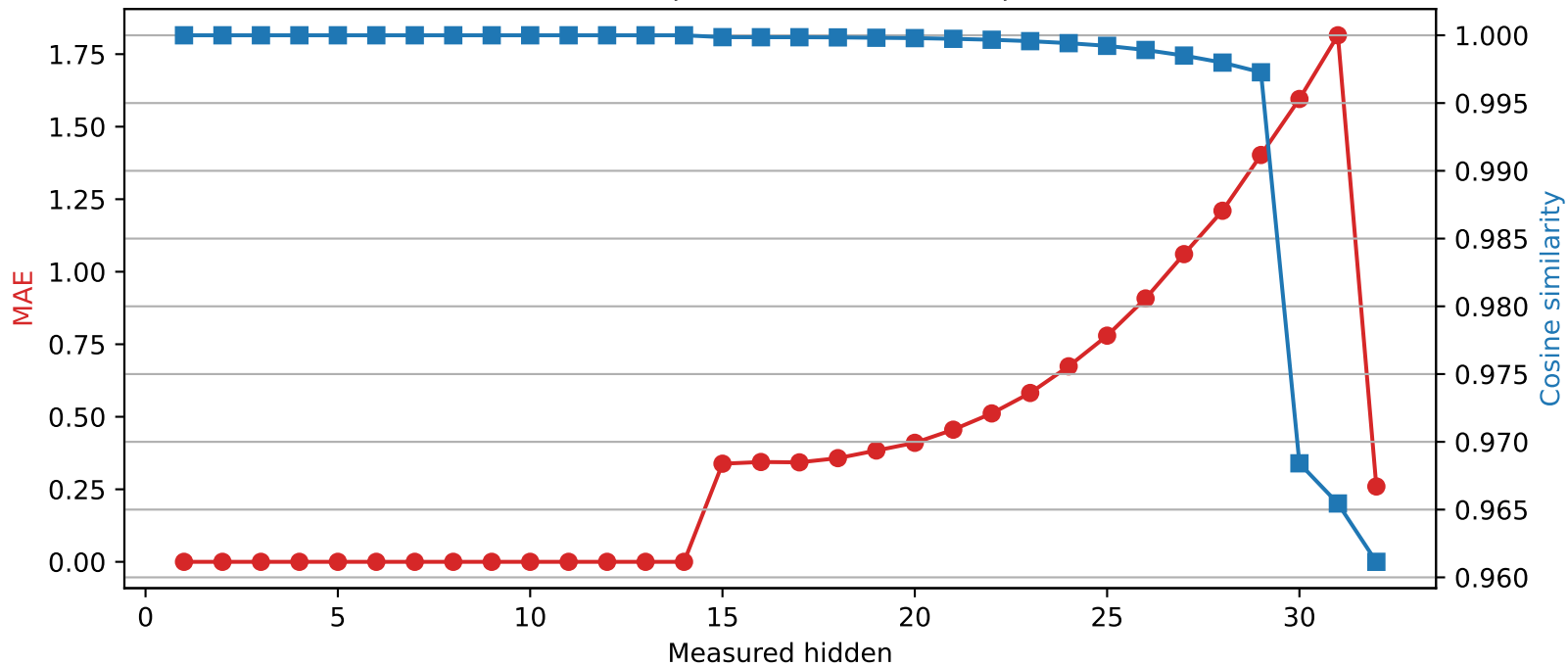
Phi-3-mini-4k-instruct | Quantized layer 14 | float64 → int4
