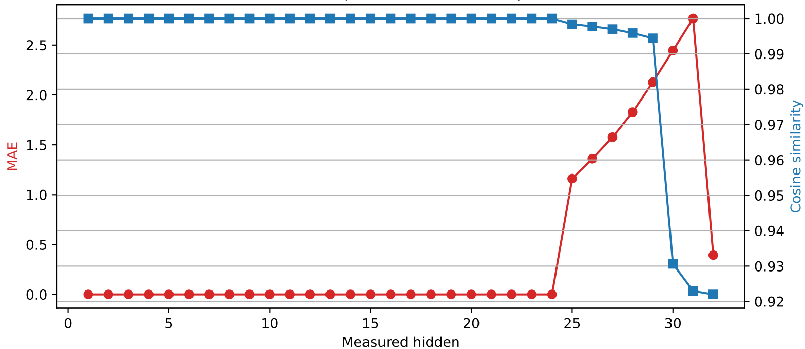
Phi-3-mini-4k-instruct | Quantized layer 24 | float64 → int4
