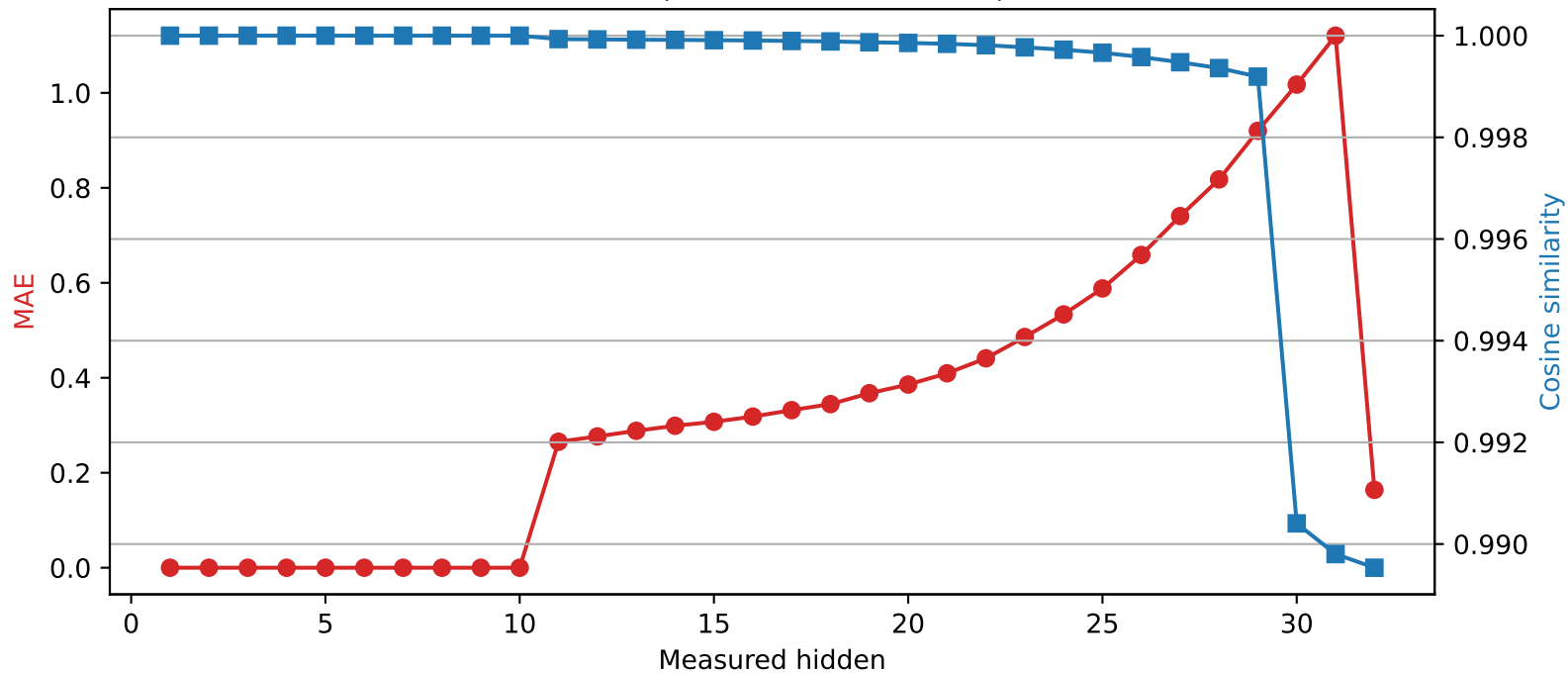
Phi-3-mini-4k-instruct | Quantized layer 10 | float64 → int4
