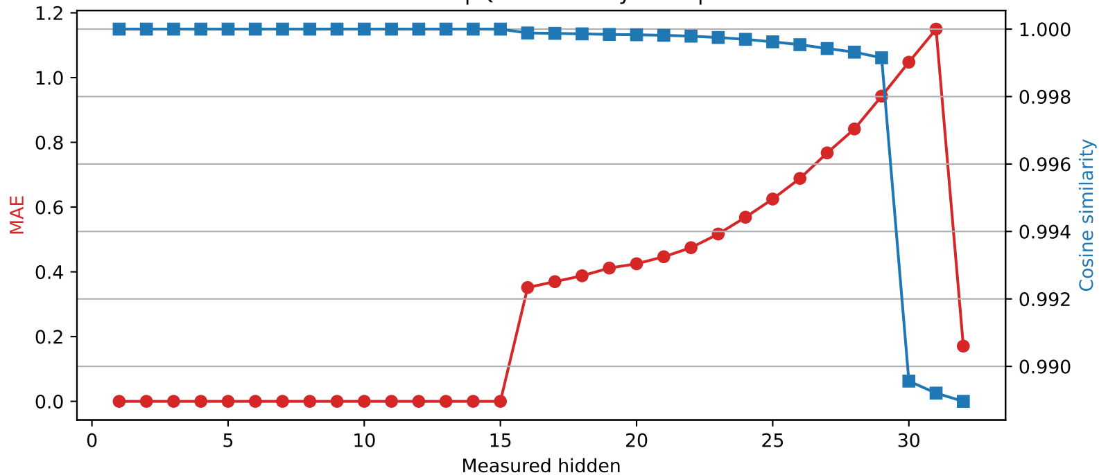
Phi-3-mini-4k-instruct | Quantized layer 15 | float64 \rightarrow int4
