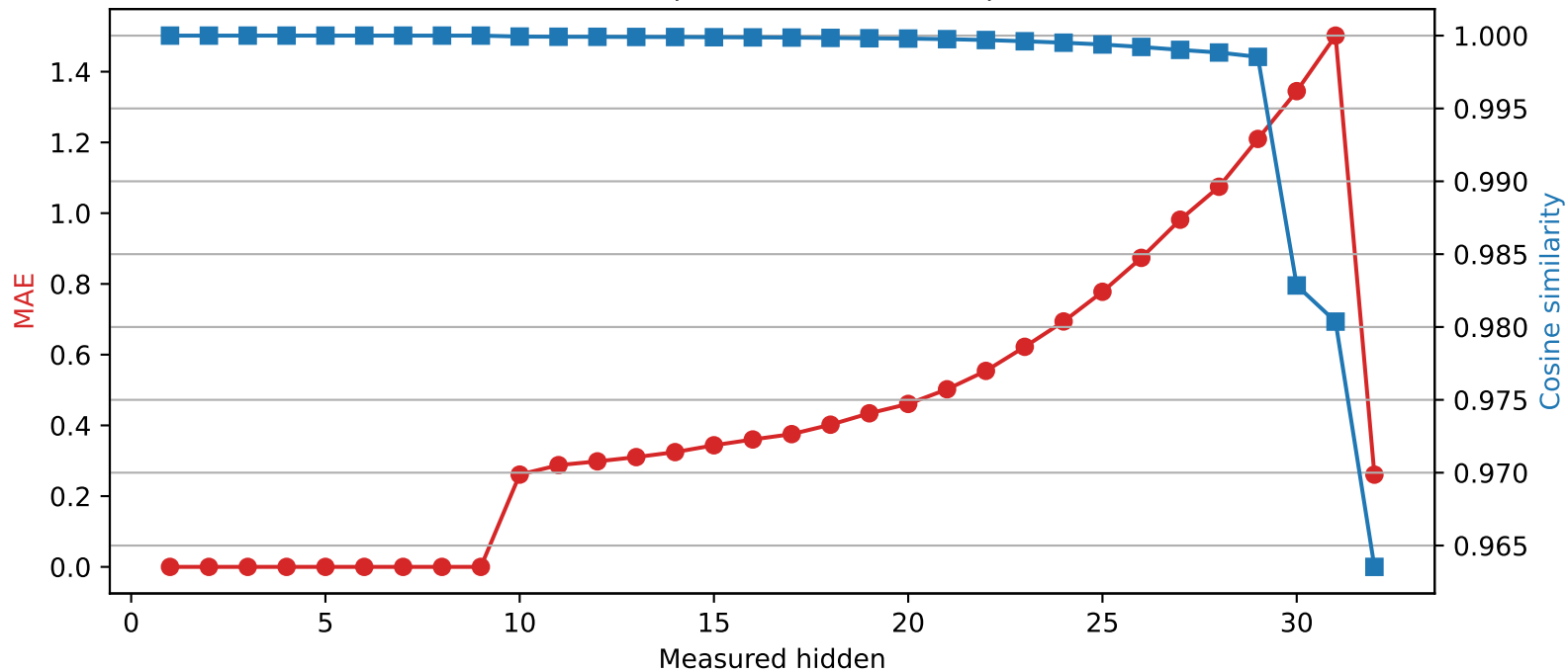
Phi-3-mini-4k-instruct | Quantized layer 9 | float64 → int4
