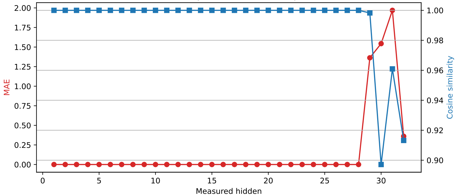
Phi-3-mini-4k-instruct | Quantized layer 28 | float64 \rightarrow int4
