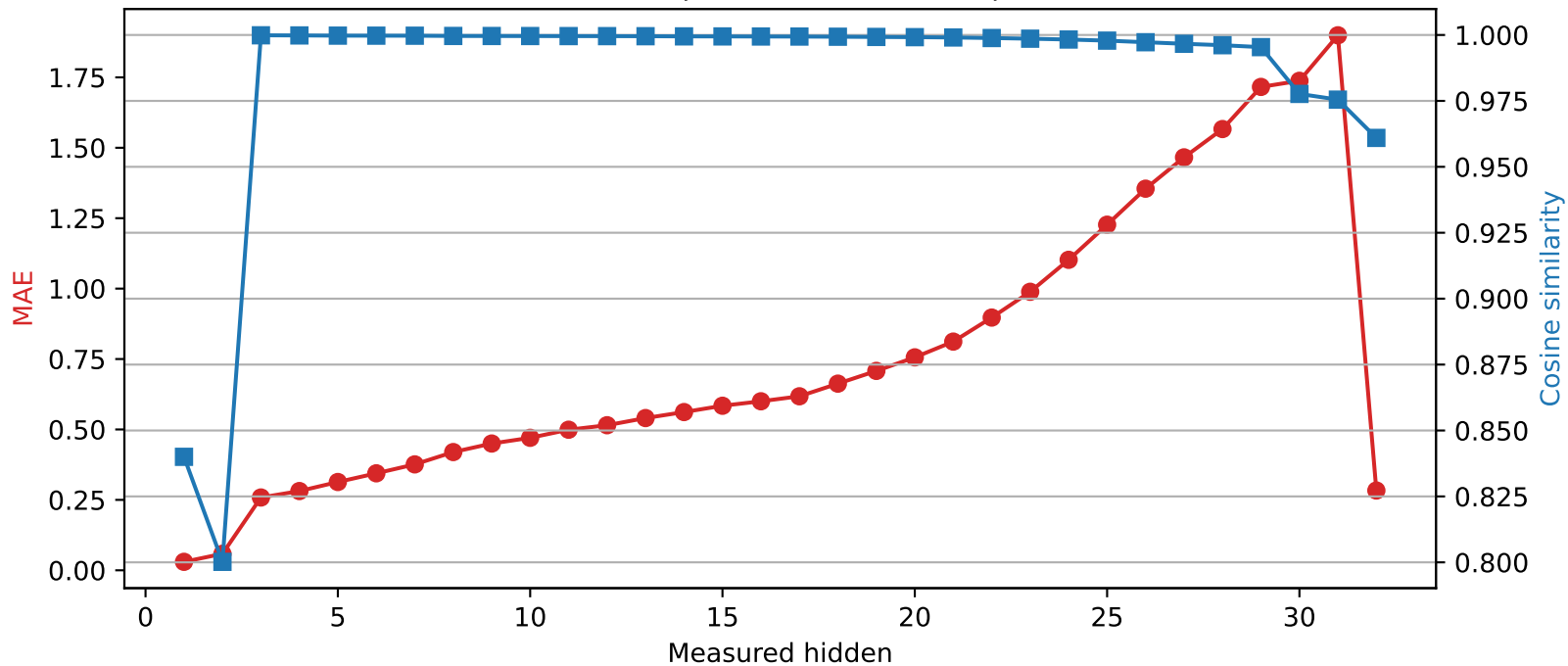
Phi-3-mini-4k-instruct | Quantized layer 0 | float64 → int4
