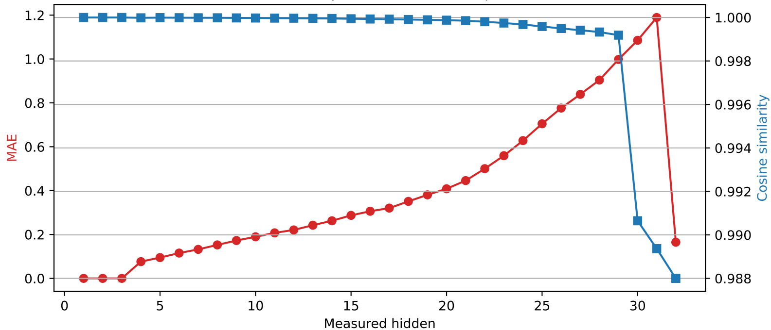
Phi-3-mini-4k-instruct | Quantized layer 3 | float64 \rightarrow int4
