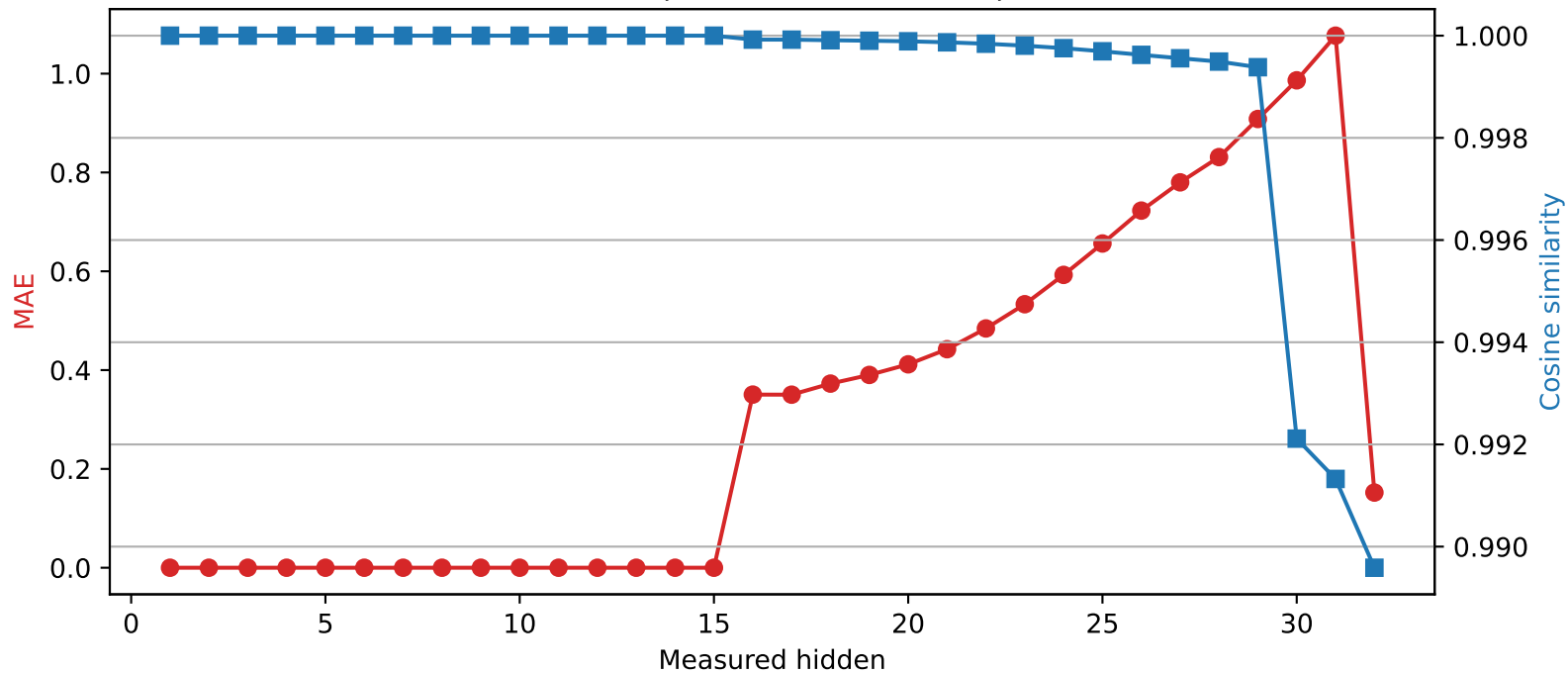
Phi-3-mini-4k-instruct | Quantized layer 15 | float64 → int4
