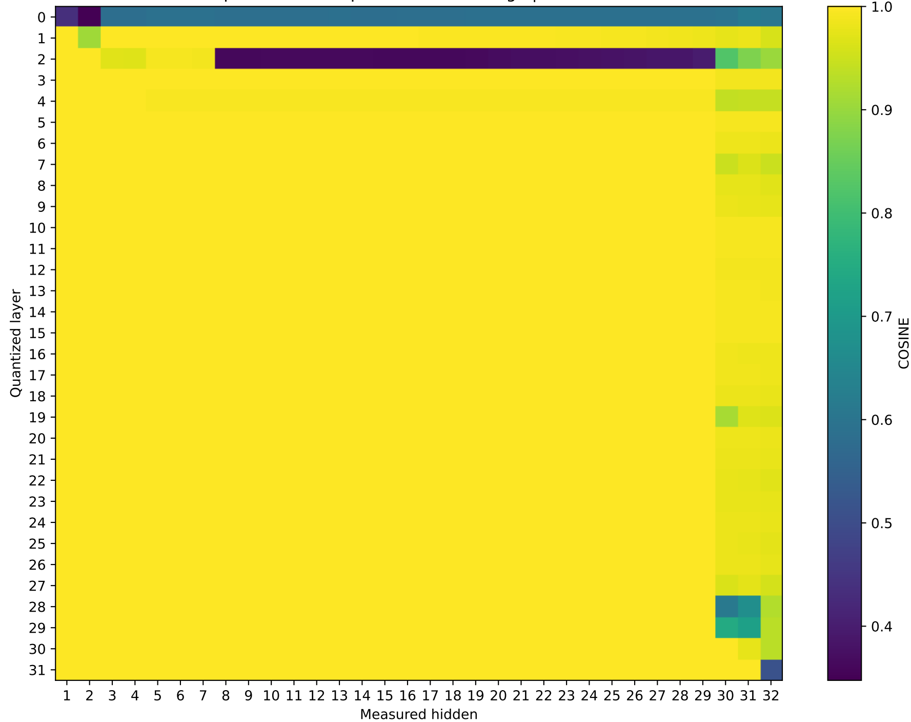
Phi-3-mini-4k-instruct Prompt 2: cos sim representation damage | float16 → int2
