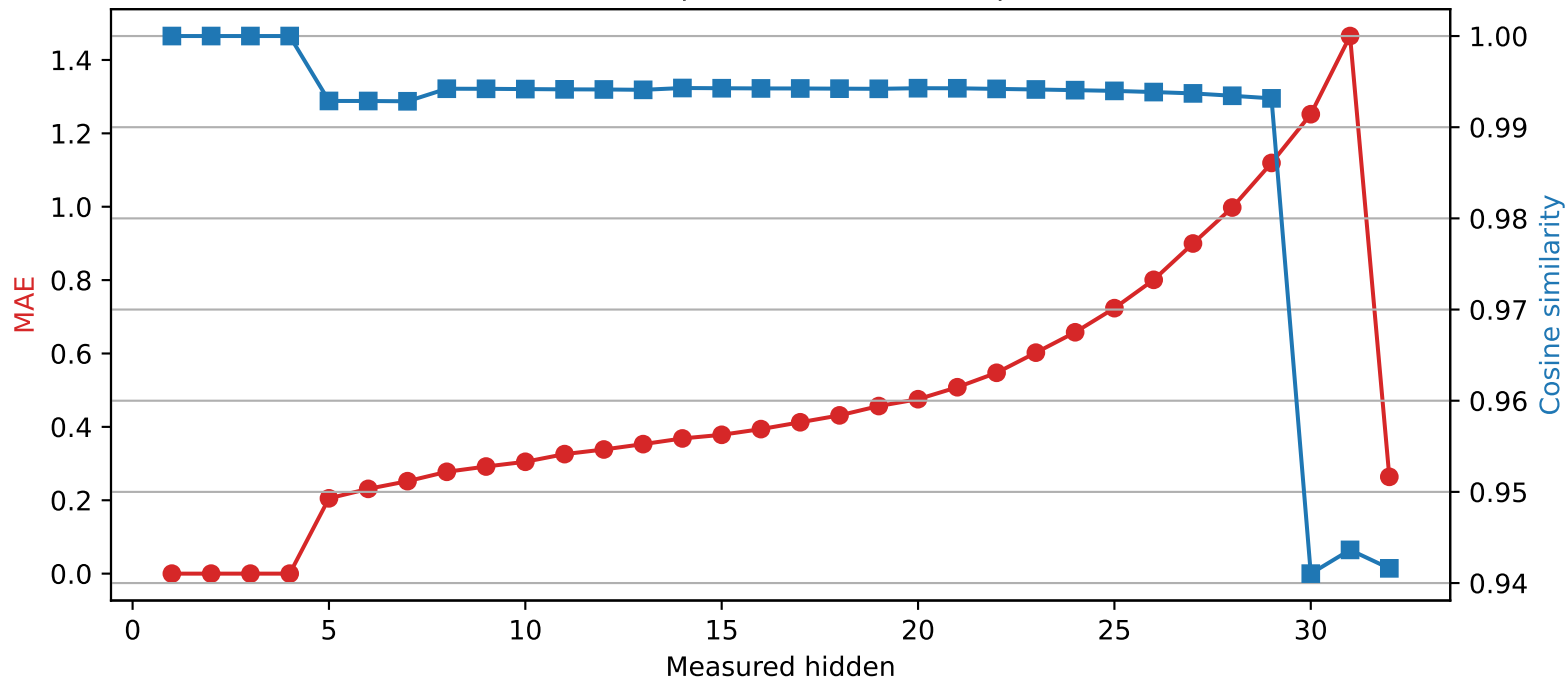
Phi-3-mini-4k-instruct | Quantized layer 4 | float16 \rightarrow int2
