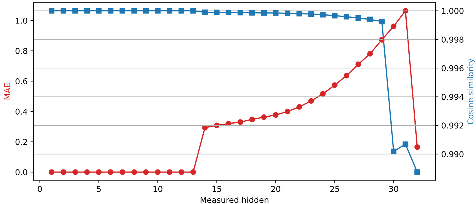
Phi-3-mini-4k-instruct | Quantized layer 13 | float16 \rightarrow int2
