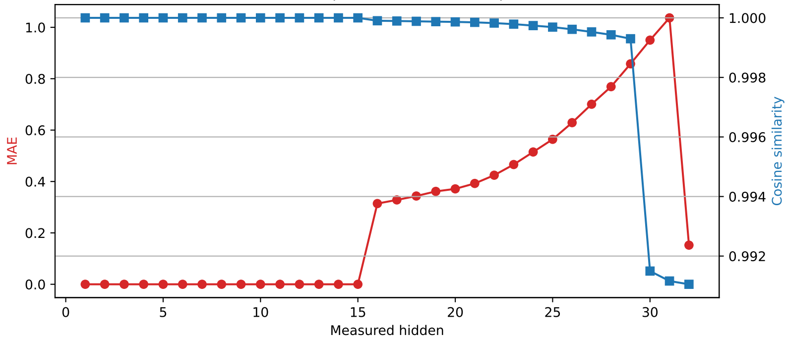
Phi-3-mini-4k-instruct | Quantized layer 15 | float16 \rightarrow int2
