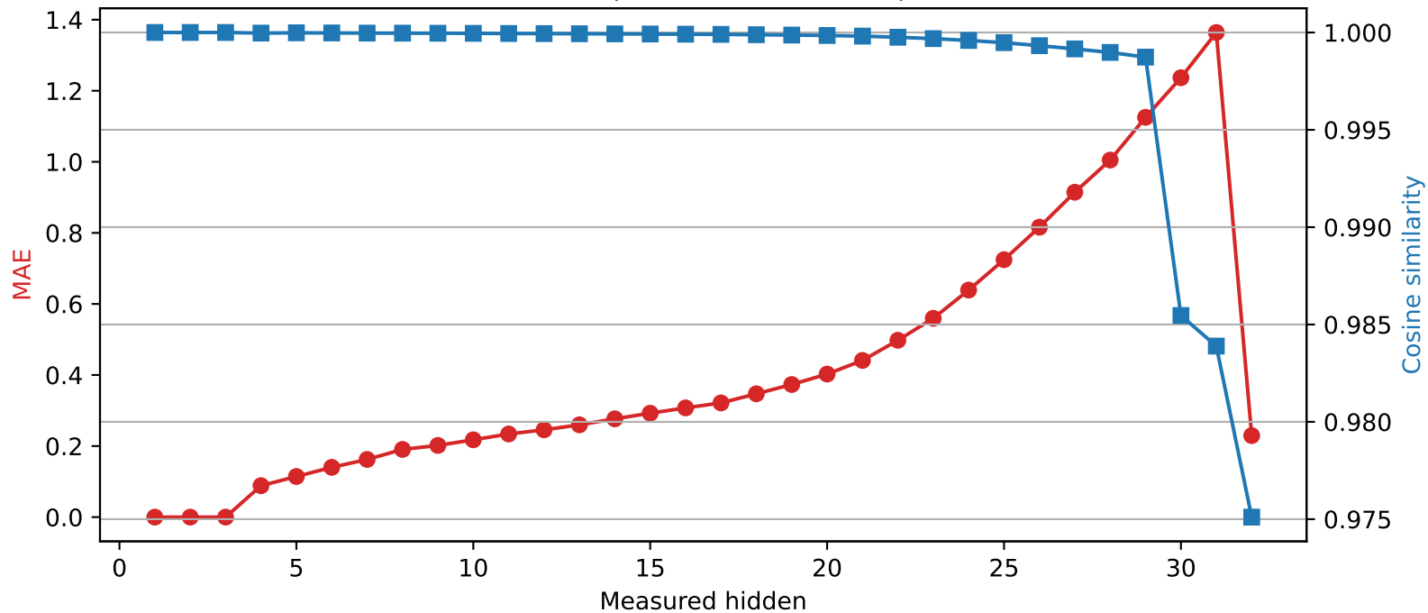
Phi-3-mini-4k-instruct | Quantized layer 3 | float16 \rightarrow int2
