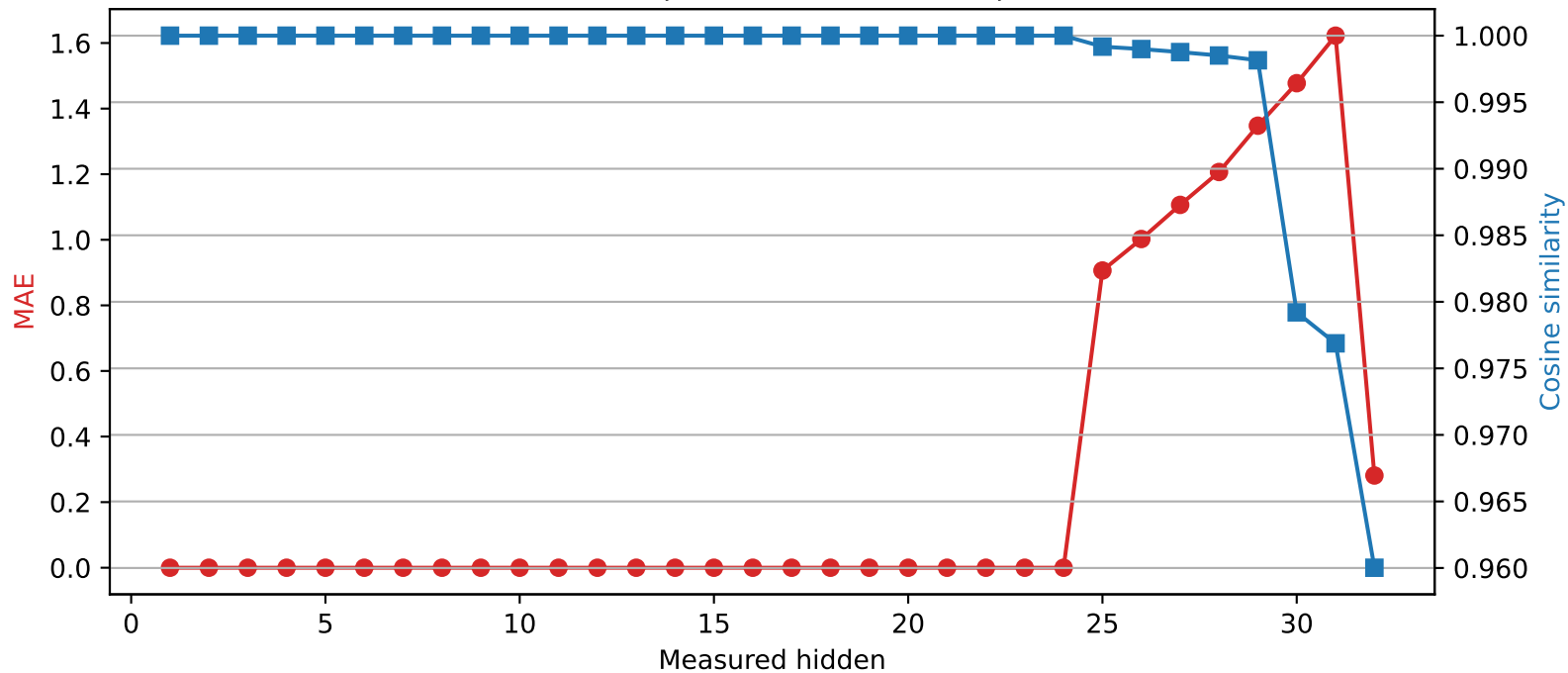
Phi-3-mini-4k-instruct | Quantized layer 24 | float16 \rightarrow int2
