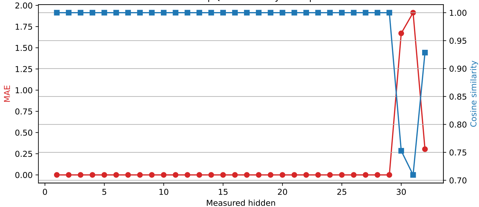
Phi-3-mini-4k-instruct | Quantized layer 29 | float16 \rightarrow int2
