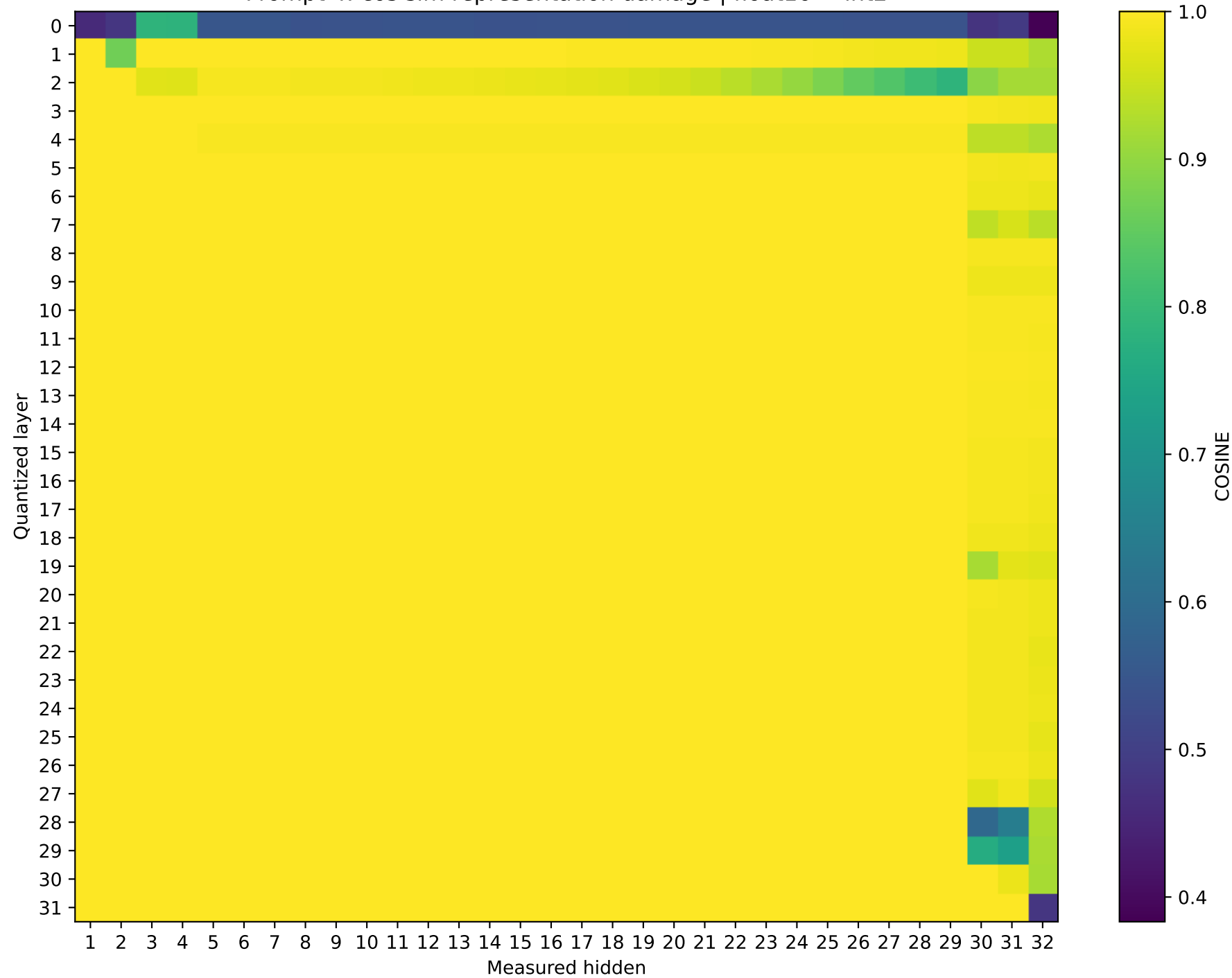
Phi-3-mini-4k-instruct Prompt 4: cos sim representation damage | float16 → int2
