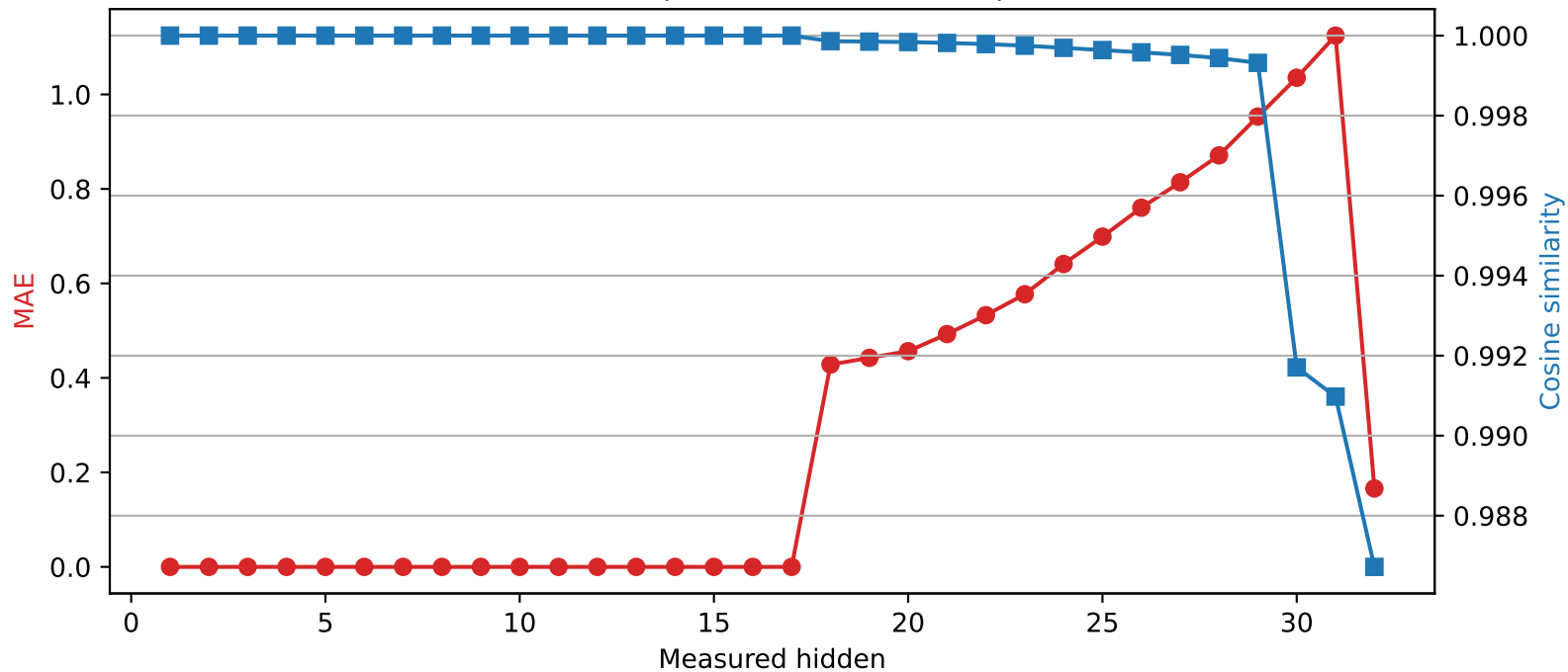
Phi-3-mini-4k-instruct | Quantized layer 17 | float16 \rightarrow int2
