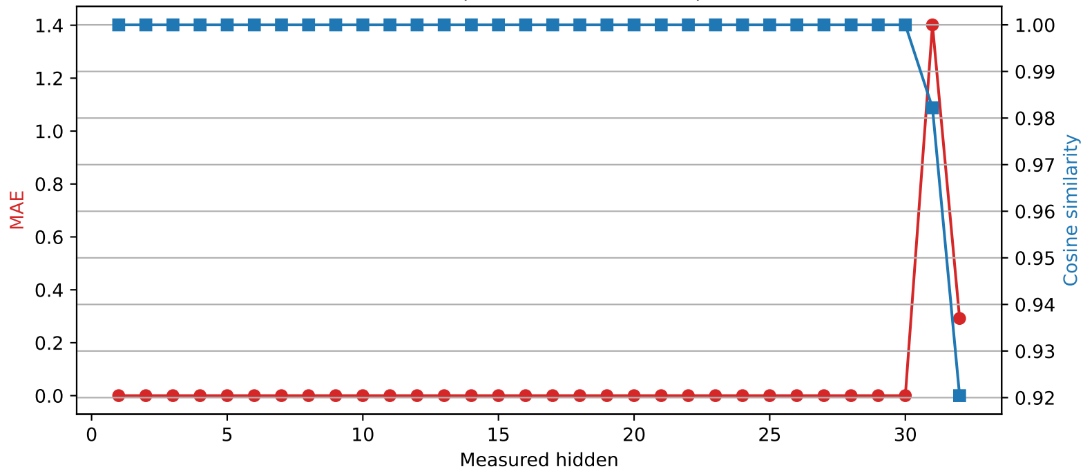
Phi-3-mini-4k-instruct | Quantized layer 30 | float16 \rightarrow int2
