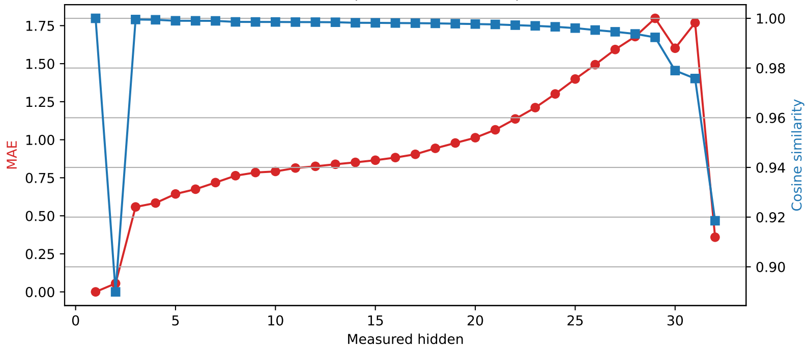
Phi-3-mini-4k-instruct | Quantized layer 1 | float32 \rightarrow int2
