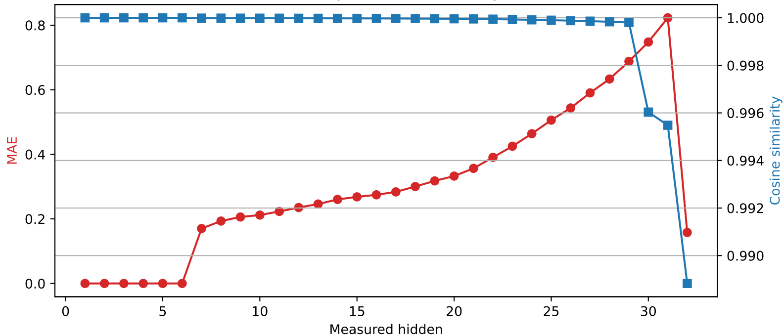
Phi-3-mini-4k-instruct | Quantized layer 6 | float32 \rightarrow int2
