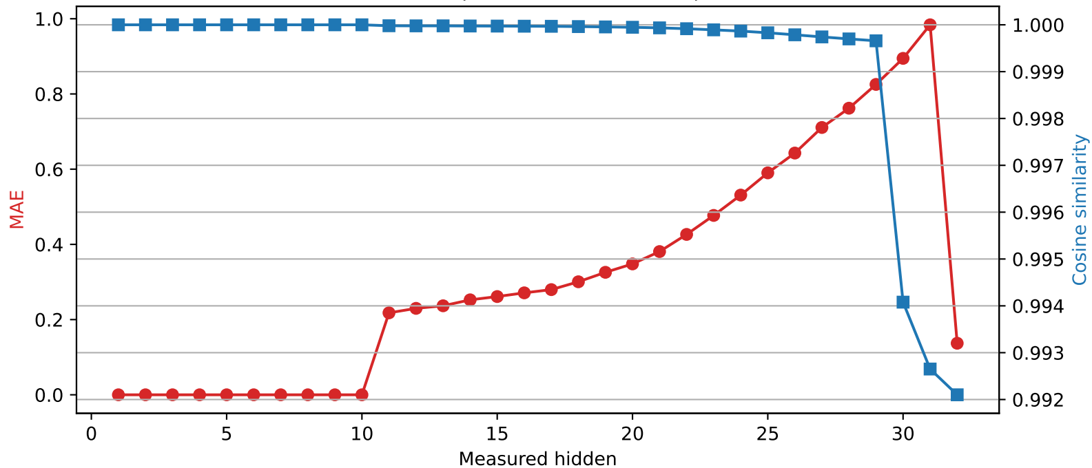
Phi-3-mini-4k-instruct | Quantized layer 10 | float32 → int2
