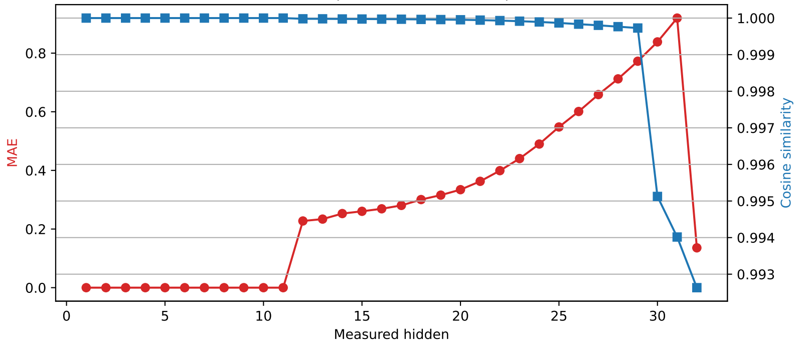
Phi-3-mini-4k-instruct | Quantized layer 11 | float32 \rightarrow int2
