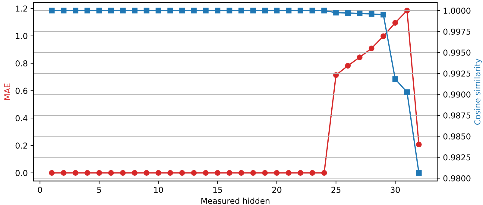
Phi-3-mini-4k-instruct | Quantized layer 24 | float32 → int2
