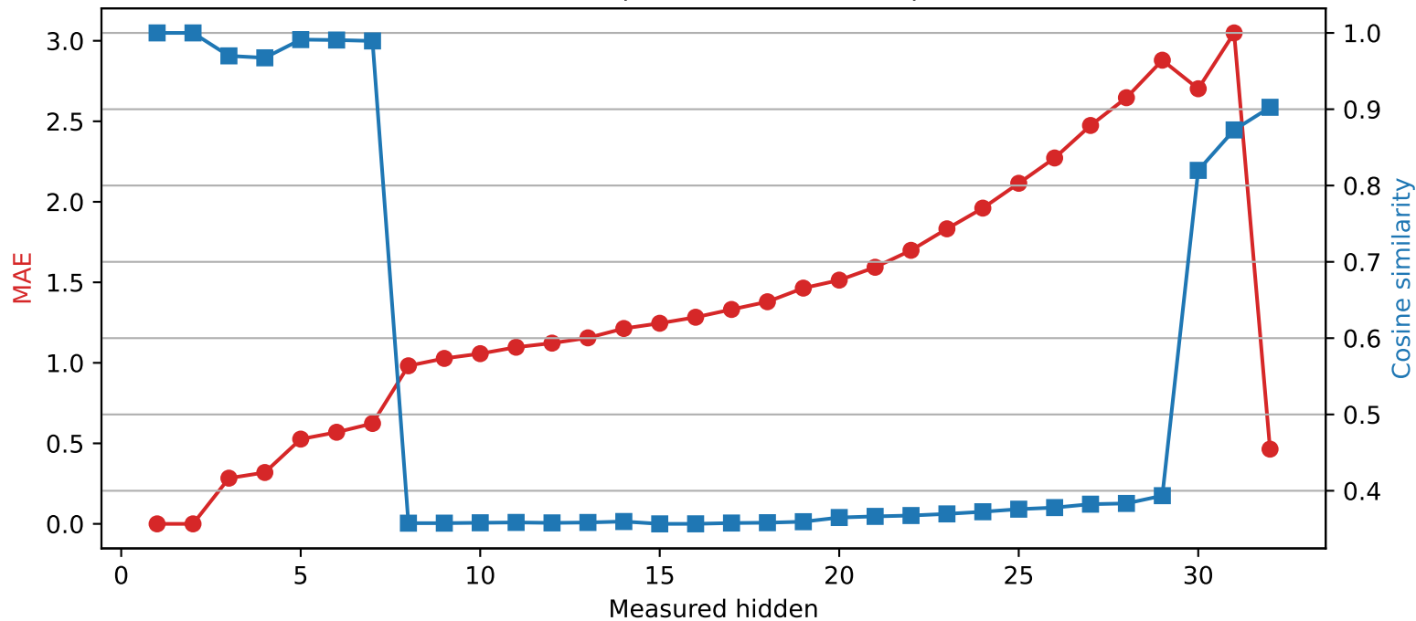
Phi-3-mini-4k-instruct | Quantized layer 2 | float32 → int2
