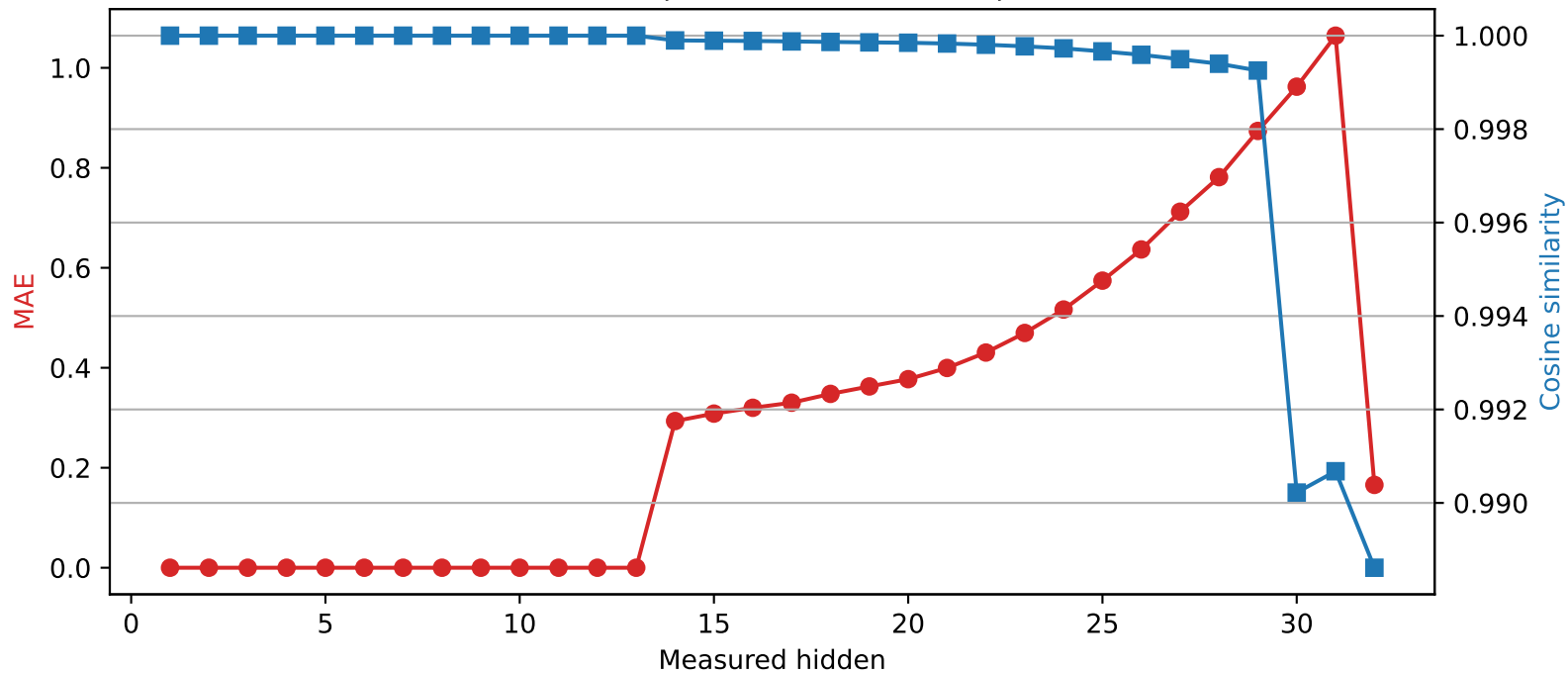
Phi-3-mini-4k-instruct | Quantized layer 13 | float32 \rightarrow int2
