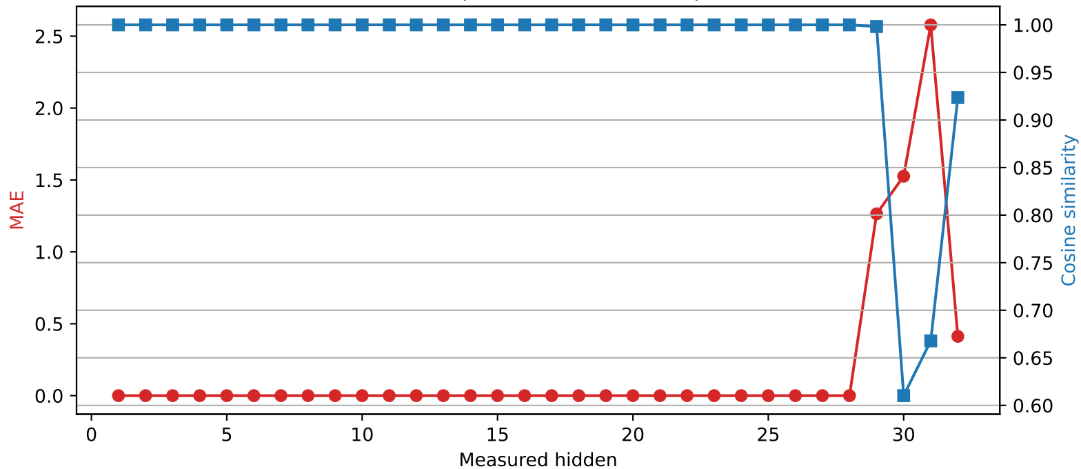
Phi-3-mini-4k-instruct | Quantized layer 28 | float32 → int2
