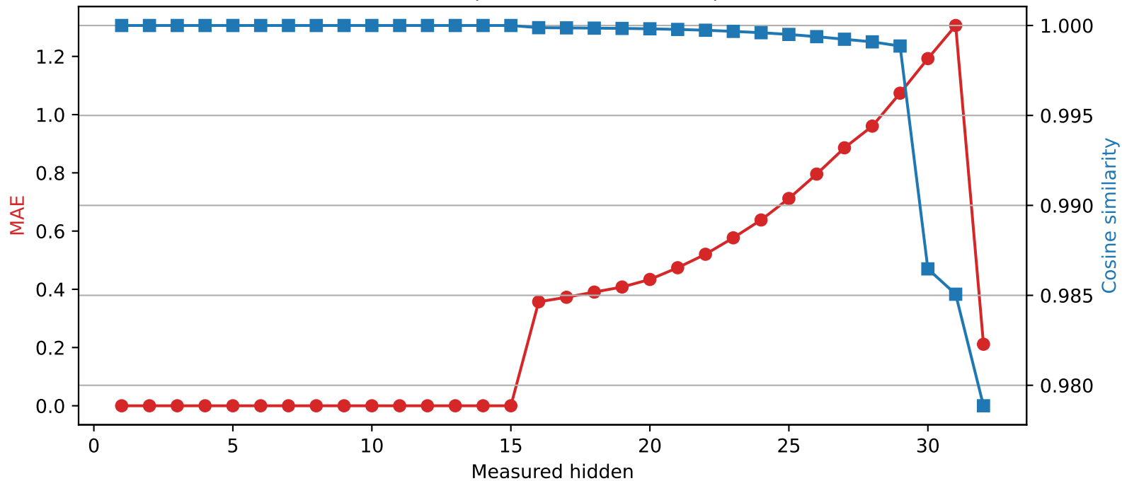
Phi-3-mini-4k-instruct | Quantized layer 15 | float32 → int2
