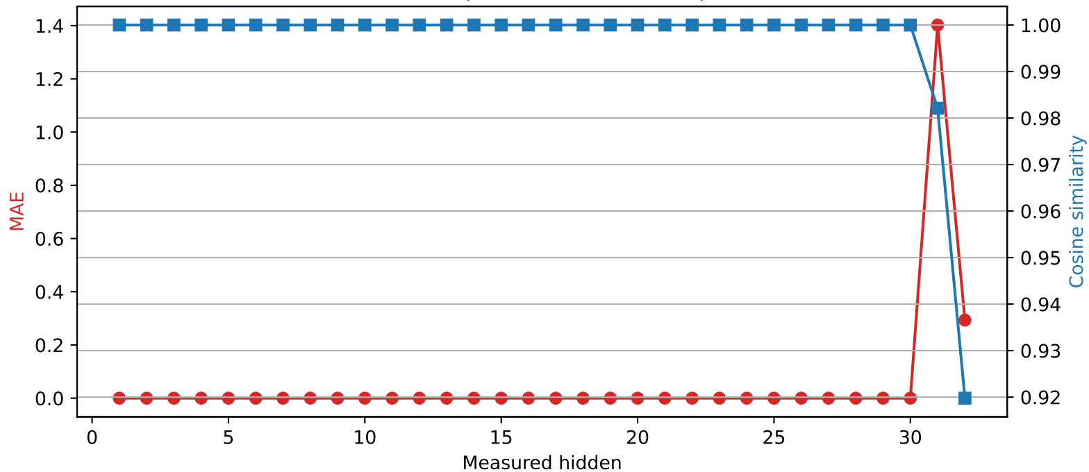
Phi-3-mini-4k-instruct | Quantized layer 30 | float32 → int2
