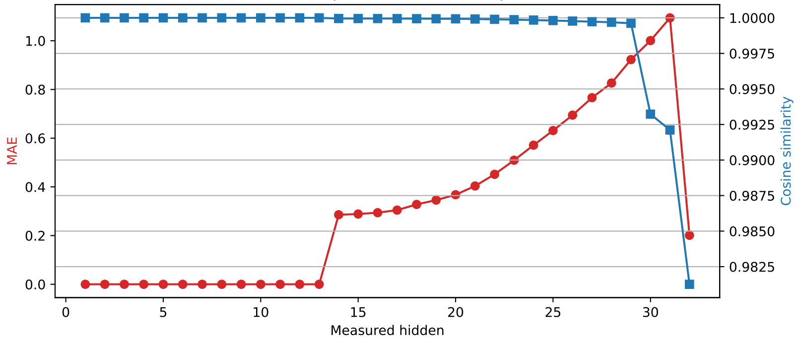
Phi-3-mini-4k-instruct | Quantized layer 13 | float64 → int2
