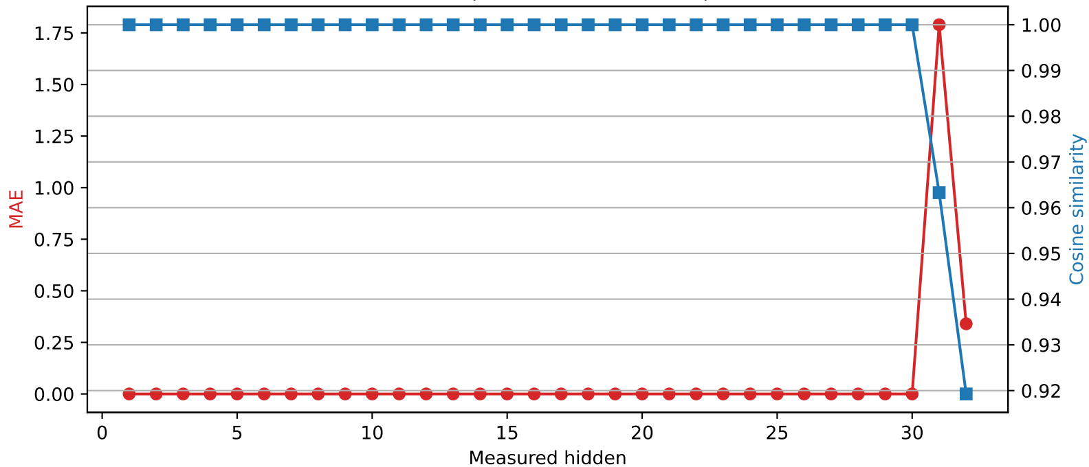
Phi-3-mini-4k-instruct | Quantized layer 30 | float64 \rightarrow int2
