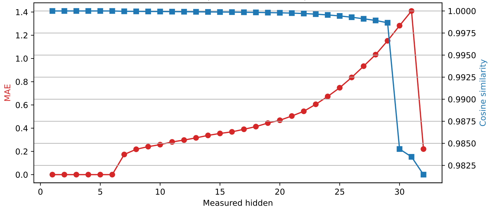
Phi-3-mini-4k-instruct | Quantized layer 6 | float64 → int2
