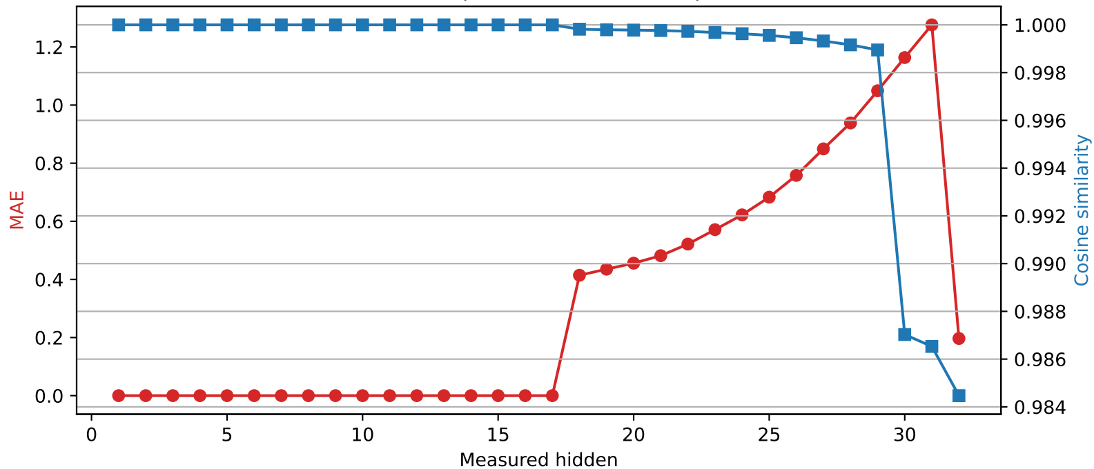
Phi-3-mini-4k-instruct | Quantized layer 17 | float64 → int2
