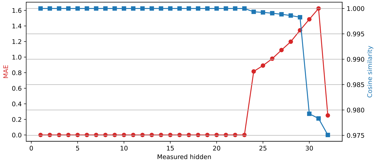
Phi-3-mini-4k-instruct | Quantized layer 23 | float64 \rightarrow int2
